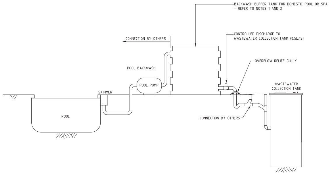
TYPICAL CONNECTION TO SWIMMING POOL ABOVE GROUND BUFFER TANK
