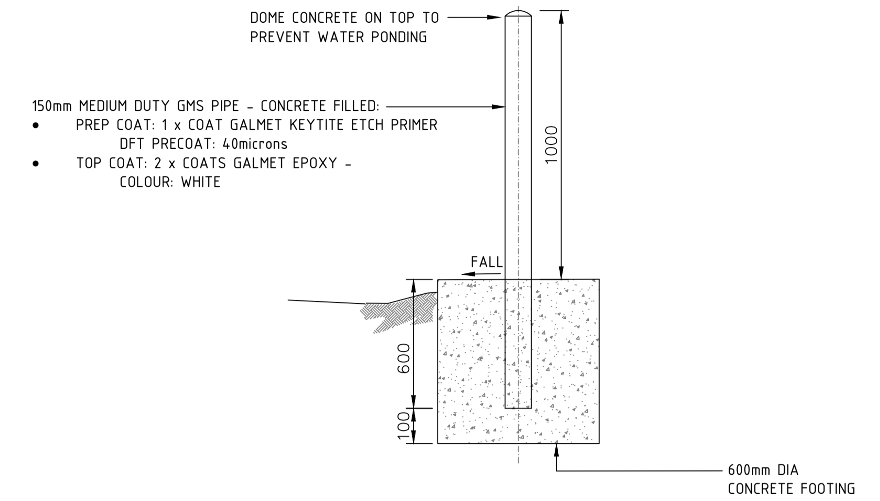
BOLLARD DETAIL
