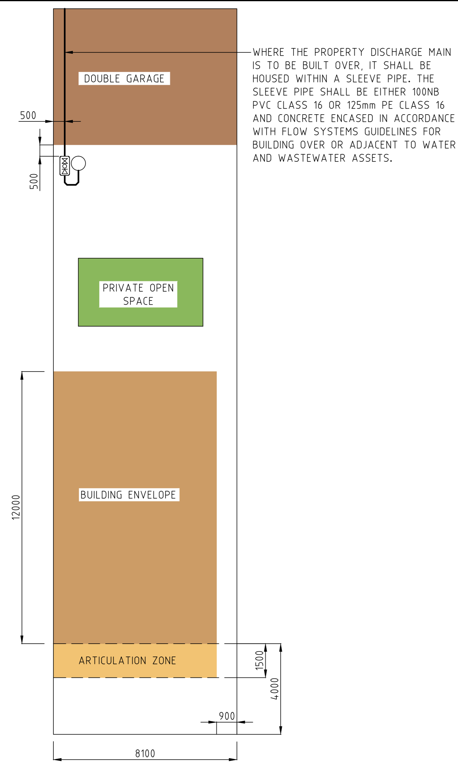
FIGURE 7 LOT TYPE: TERRACE / ABUTTING LOT - REAR LOADED - LOT SIZE = APPROX 200m 2 to 350m 2 NOTE: PROPERTY AND BUILDING DIMENSIONS ARE INDICATIVE ONLY.
