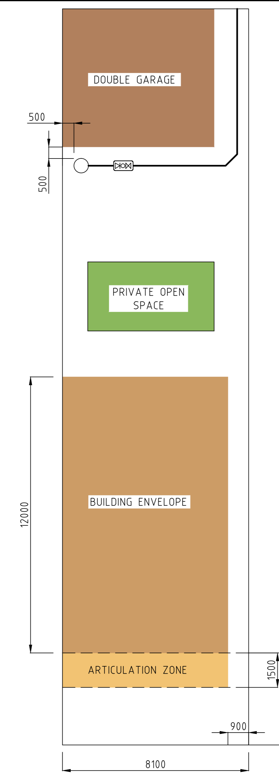
FIGURE 8 LOT TYPE: TERRACE / ABUTTING LOT - REAR LOADED - LOT SIZE = APPROX 250m 2 to 350m 2 NOTE: PROPERTY AND BUILDING DIMENSIONS ARE INDICATIVE ONLY.
