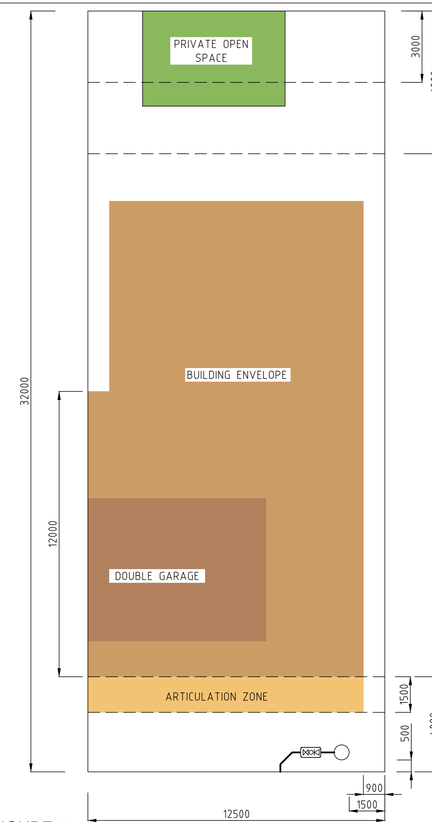
FIGURE 10 LOT TYPE: TRANSITION DWELLING - FRONT LOADED - LOT SIZE = APPROX 400m 2 NOTE: PROPERTY AND BUILDING DIMENSIONS ARE INDICATIVE ONLY.
